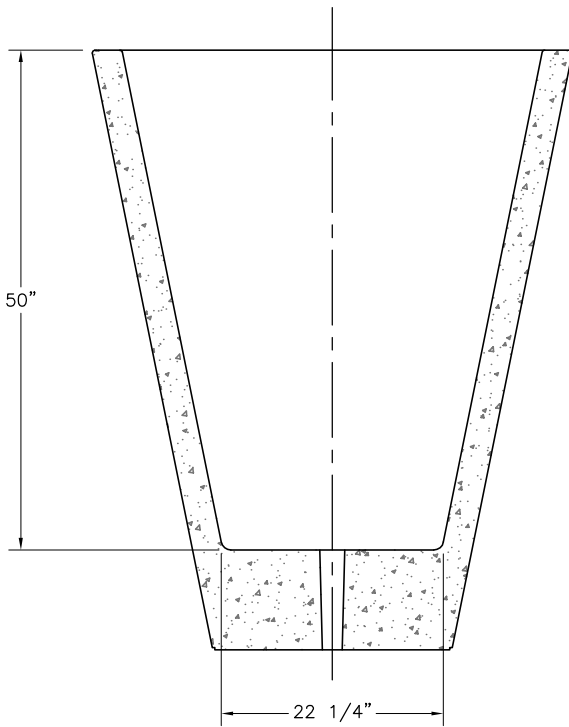
SECTION VIEW
