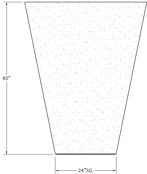
ELEVATION VIEW
