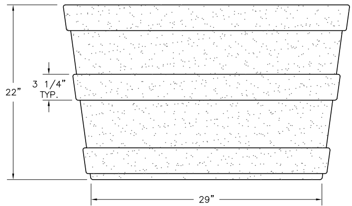
ELEVATION VIEW
