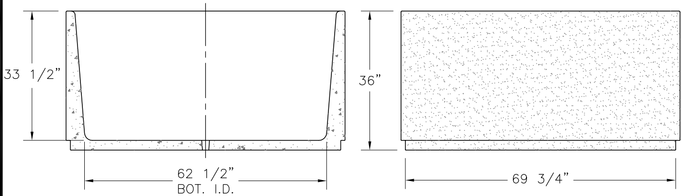
SECTION VIEW
