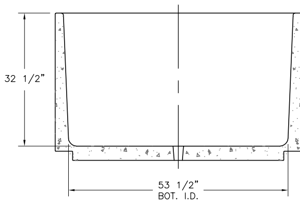
SECTION VIEW
