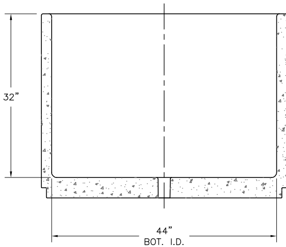
SECTION VIEW
