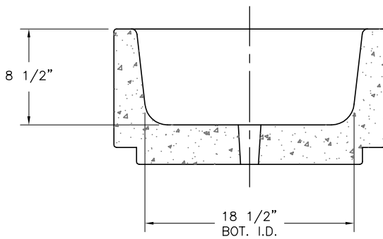
SECTION VIEW
