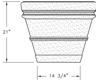
ELEVATION VIEW
