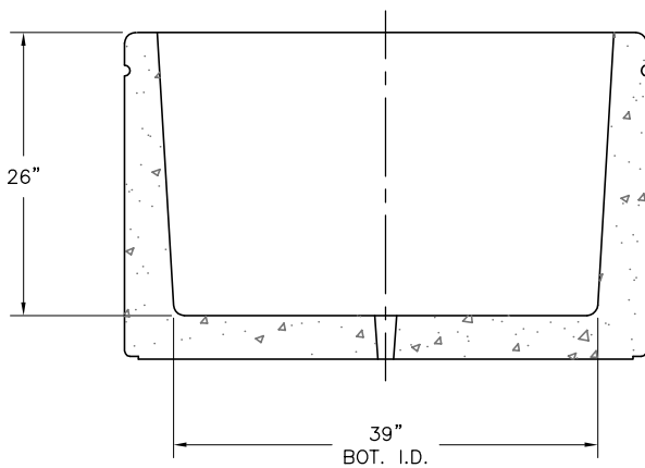
SECTION VIEW
