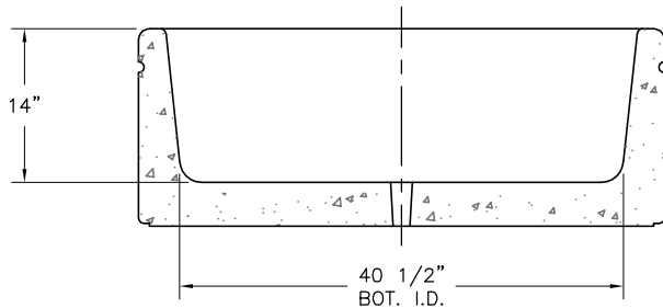
SECTION VIEW
