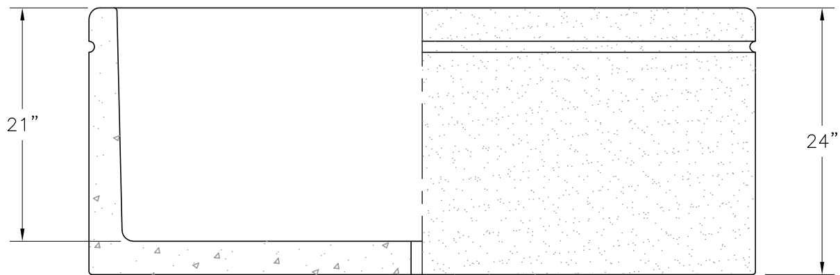
SECTION/ELEVATION VIEW
