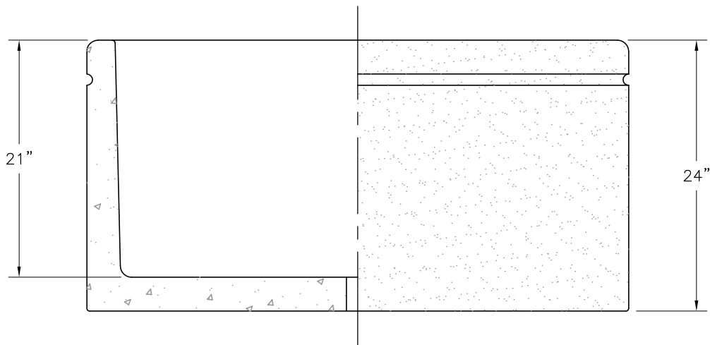
SECTION/ELEVATION VIEW
