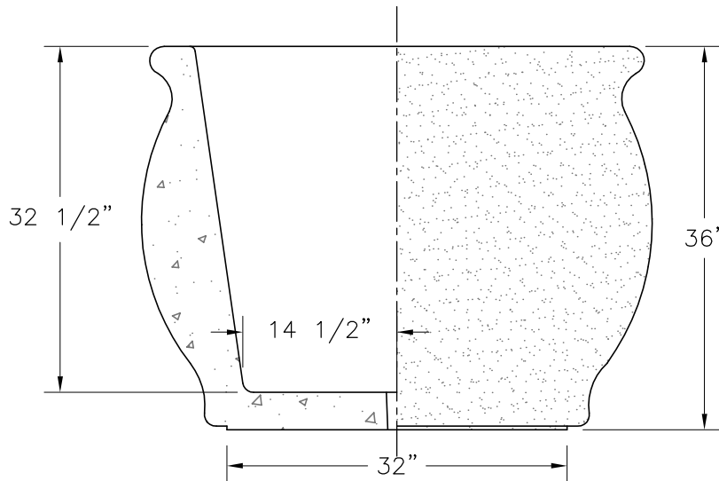
SECTION/ELEVATION VIEW
