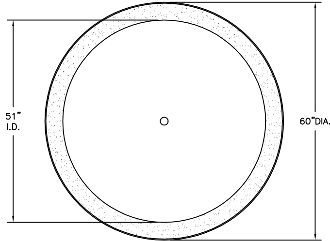
PLAN VIEW
