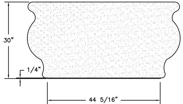
ELEVATION VIEW
