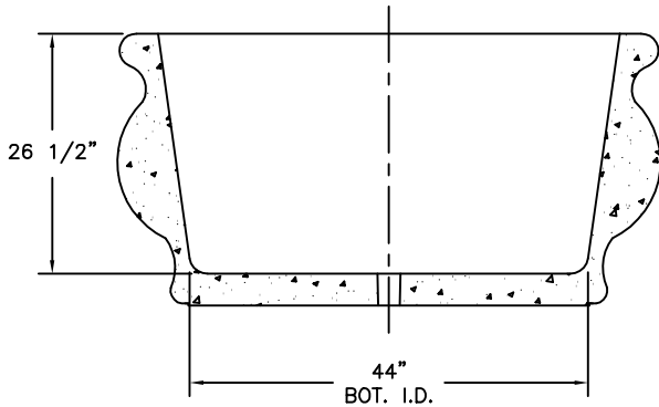
SECTION VIEW
