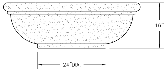
ELEVATION VIEW
