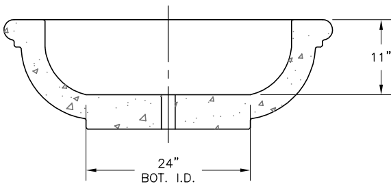
SECTION VIEW
