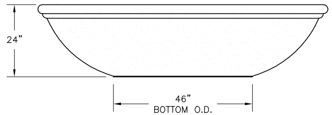
ELEVATION VIEW
