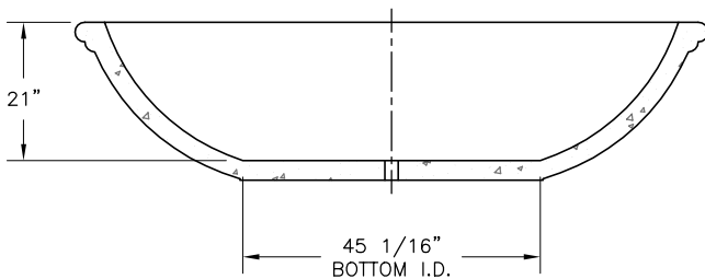
SECTION VIEW
