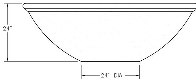
ELEVATION VIEW
