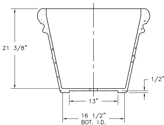
SECTION VIEW
