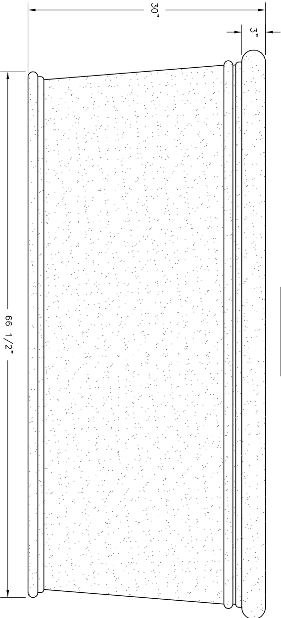
ELEVATION VIEW
