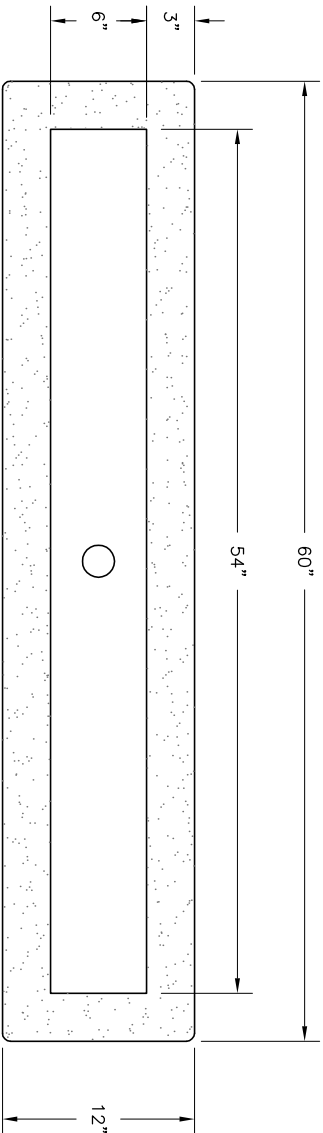
PLAN VIEW
