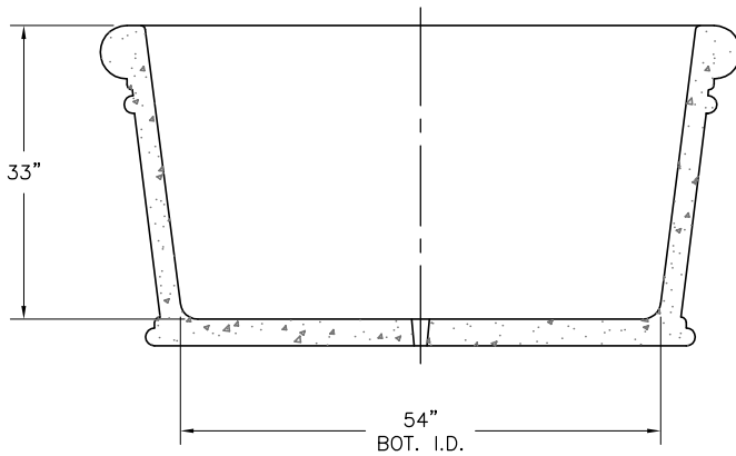
SECTION VIEW
