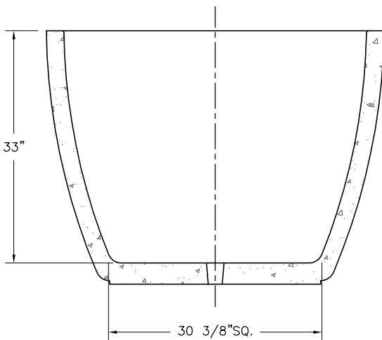
SECTION VIEW
