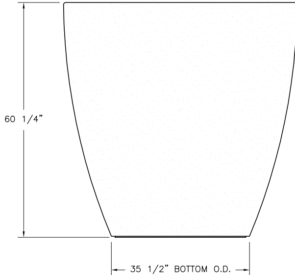
ELEVATION VIEW
