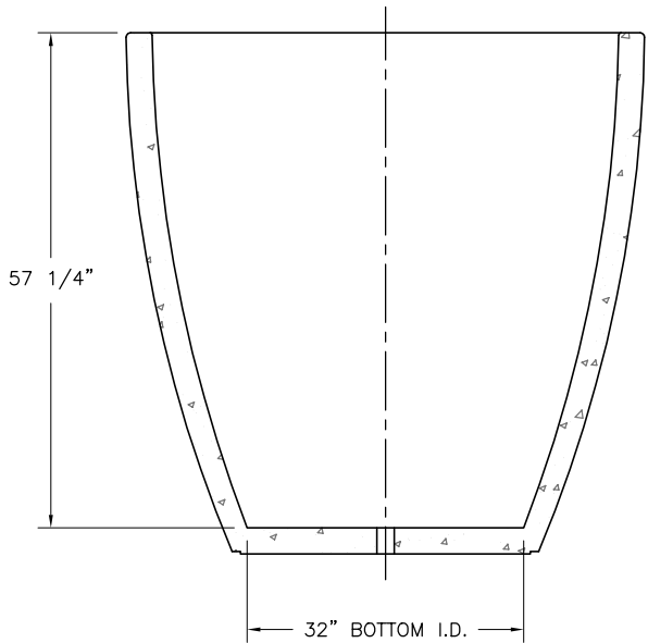
SECTION VIEW
