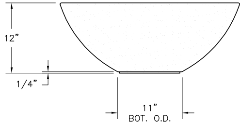
ELEVATION VIEW
