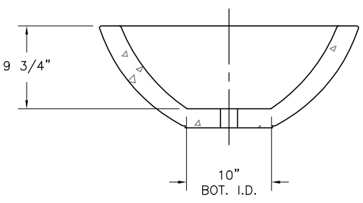
SECTION VIEW
