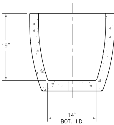
SECTION VIEW
