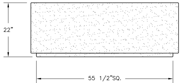
ELEVATION VIEW
