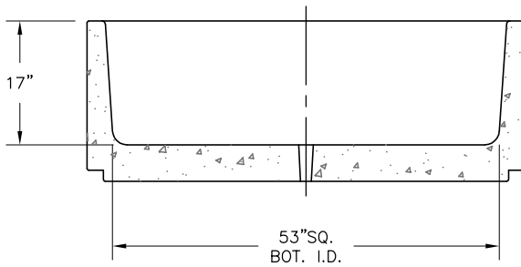
SECTION VIEW
