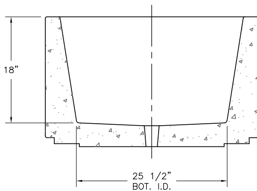
SECTION VIEW
