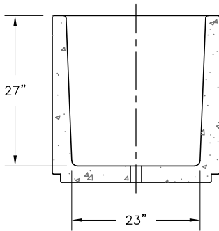
SECTION VIEW
