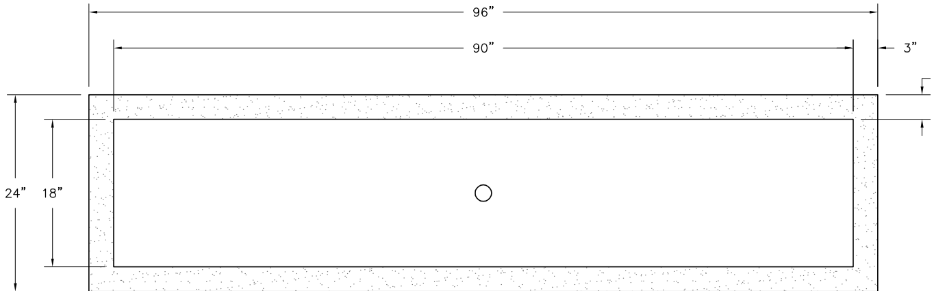
PLAN VIEW
