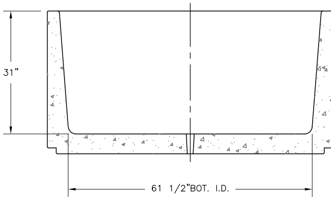
SECTION VIEW
