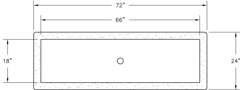
PLAN VIEW
