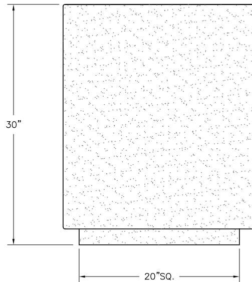
ELEVATION VIEW
