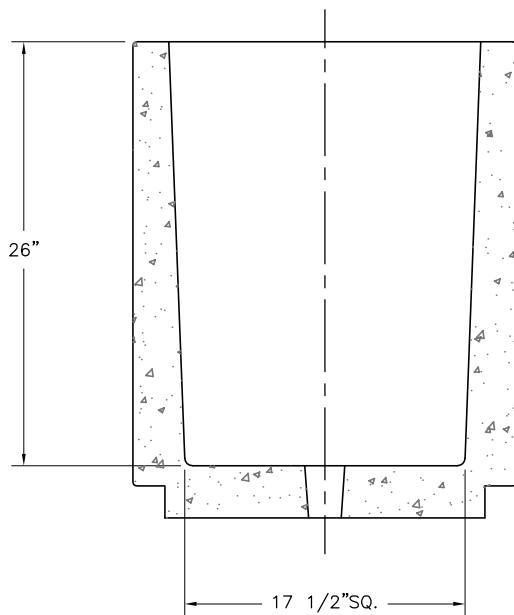
SECTION VIEW
