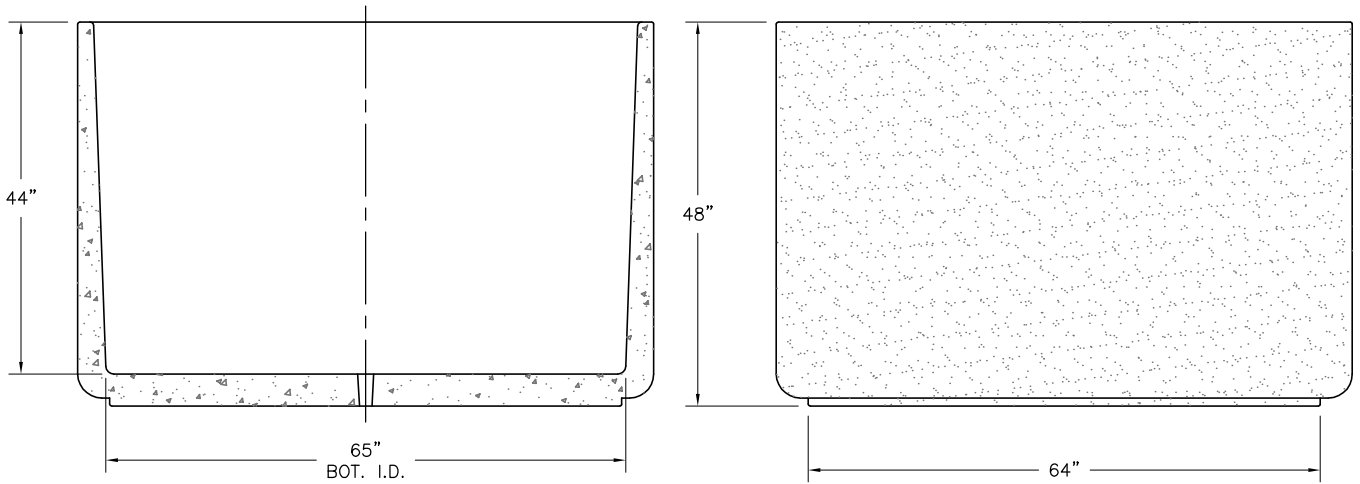
SECTION VIEW
