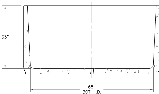
SECTION VIEW
