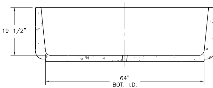
SECTION VIEW
