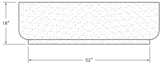
ELEVATION VIEW
