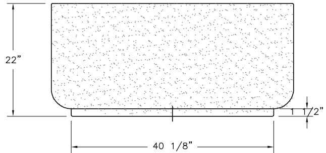
ELEVATION VIEW
