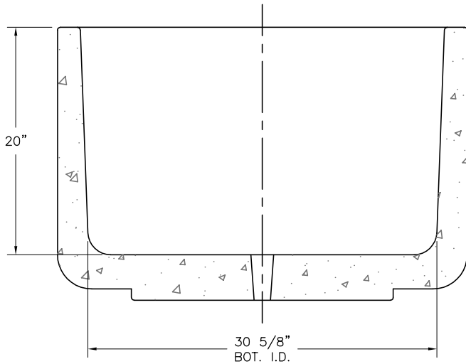
SECTION VIEW
