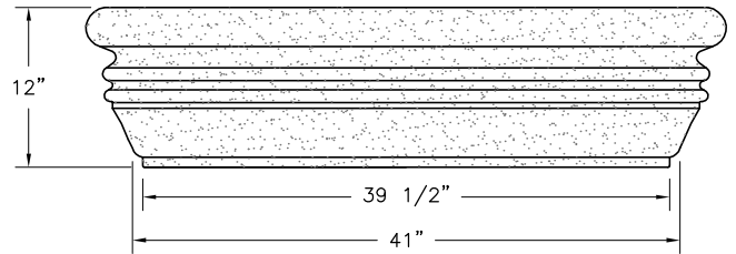
ELEVATION VIEW
