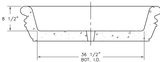
SECTION VIEW
