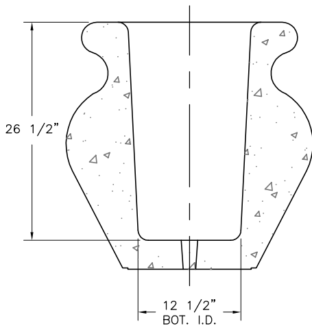
SECTION VIEW
