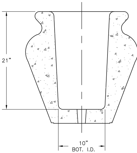
SECTION VIEW
