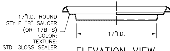
ELEVATION VIEW
